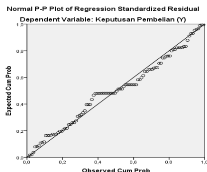
Gambar 2. Normal Probability Plot
