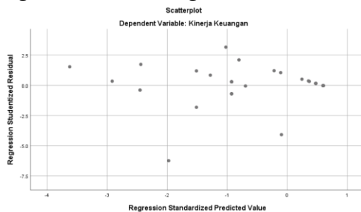
Gambar 2. Scatterplot
