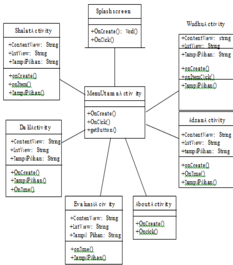
Gambar 4. Class Diagram
