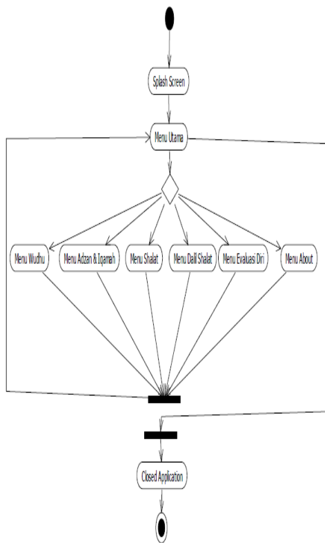
Gambar 5. Activity Diagram
