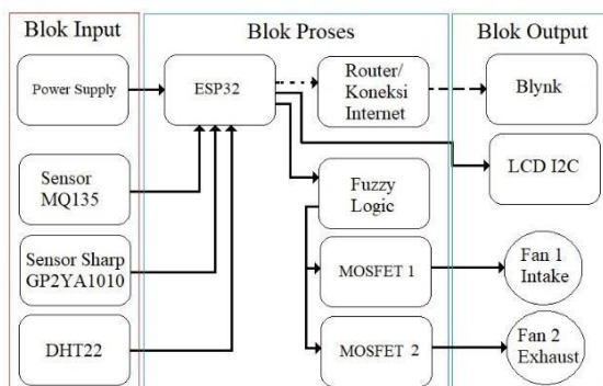
Gambar 2. Blok Diagram System
