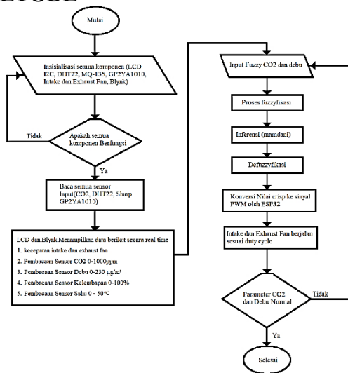
Gambar 1. Flowchart System
