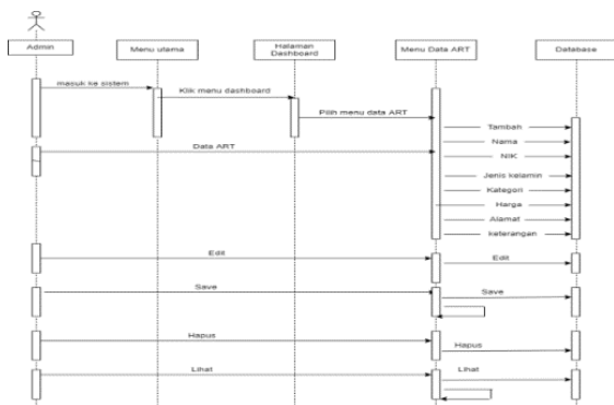
Gambar 19. Sequence Diagram Data ART
