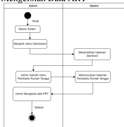
Gambar 9. Activity Diagram Mengelola Data ART
