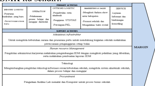
Gambar 2. Value Chain
