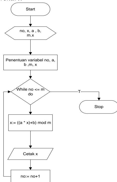
Gambar. 2 Flowchart Linear Congruent Generators
