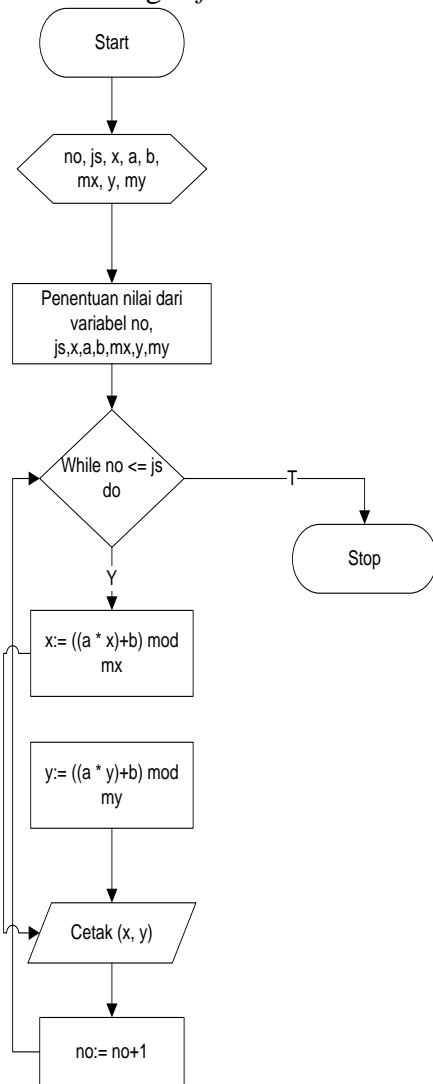
Gambar. 3 Flowchart Coupled Linear Congruent Generators
